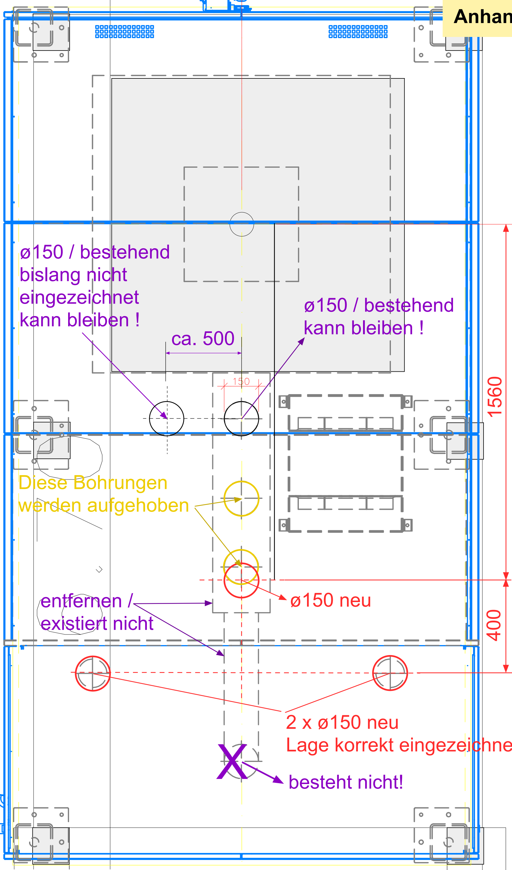
Grundriss Sockelgeschoss Krematorium Olten
